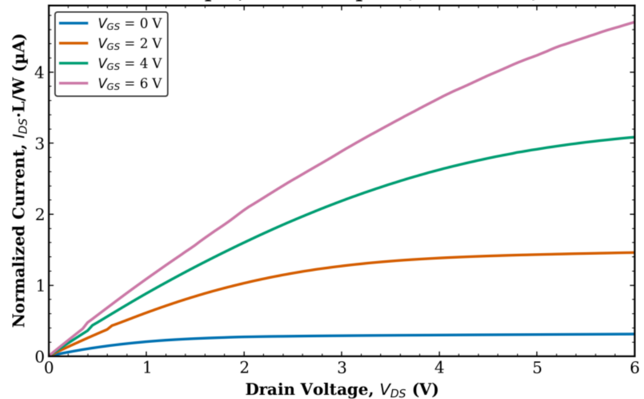
TFT3 Combined (Tr. 1 & 2) L = 8 \mu\text{m} , W = 100 \mu\text{m} (normalized)
