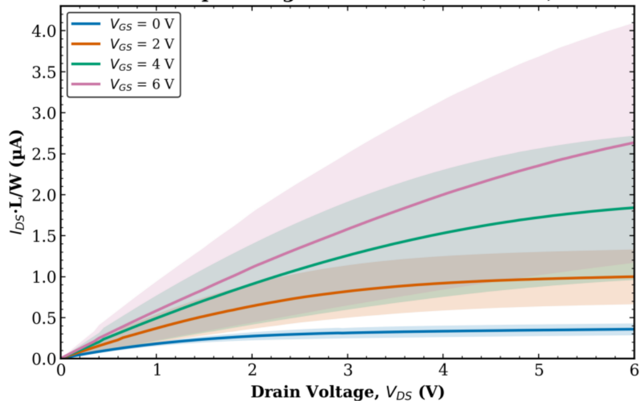
TFT3 Combined (Tr. 1 & 2) L = 8 \mu\text{m} - avg over all W (mean \pm std)
