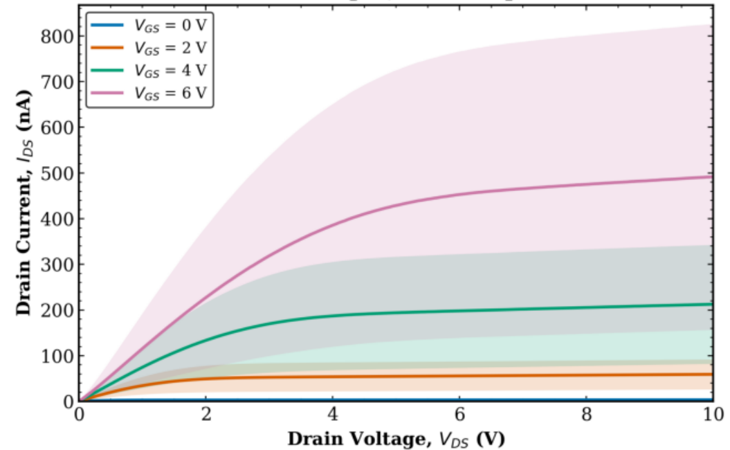
TFT3 Combined (Tr. 1 & 2) L = 160 \mu\text{m} , W = 10 \mu\text{m}
