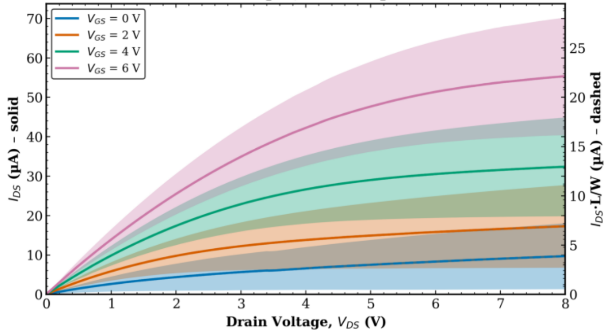
TFT3 Combined (Tr. 1 & 2) L = 20 \mu\text{m} , W = 50 \mu\text{m}
