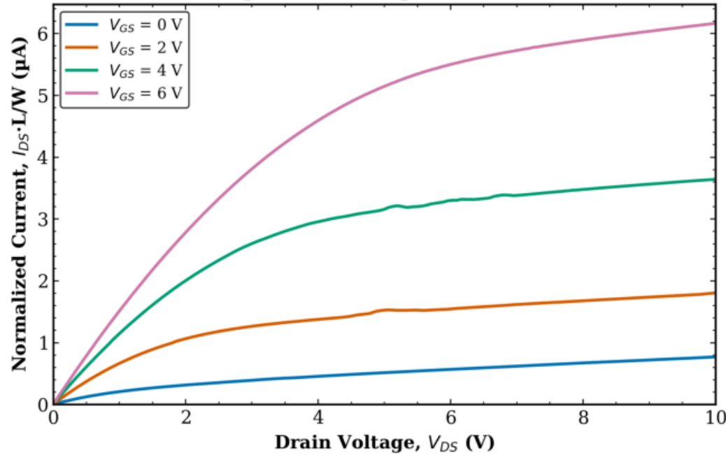
TFT3 Combined (Tr. 1 & 2) L = 10 \mu\text{m} , W = 50 \mu\text{m} (normalized)
