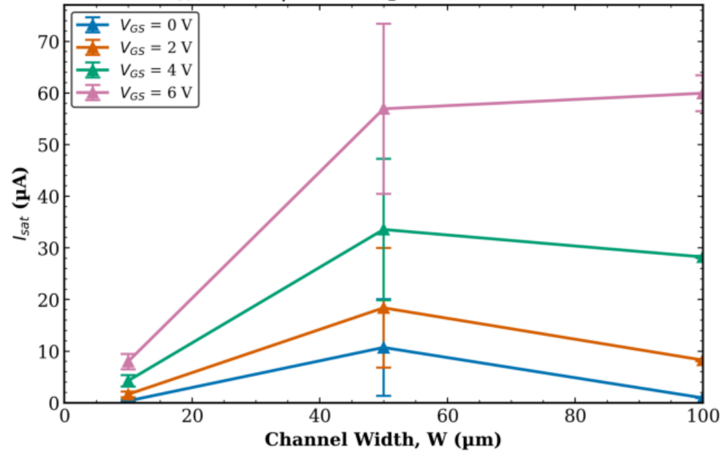
TFT3 Combined (Tr. 1 & 2) I_{sat} vs W | L = 20 μm (mean \pm std)
