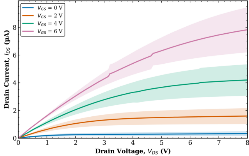
TFT3 Combined (Tr. 1 & 2) L = 20 \mu\text{m} , W = 10 \mu\text{m}
