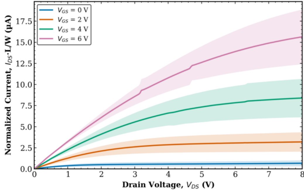
TFT3 Combined (Tr. 1 & 2) L = 20 \mu\text{m} , W = 10 \mu\text{m} (normalized)
