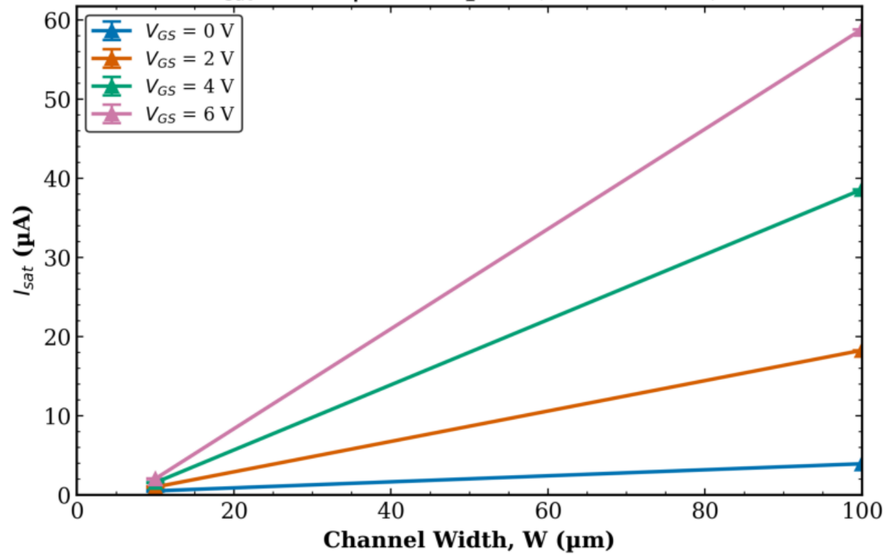
TFT3 Combined (Tr. 1 & 2) I_{sat} vs W | L = 8 \mu\text{m} (mean \pm std)
