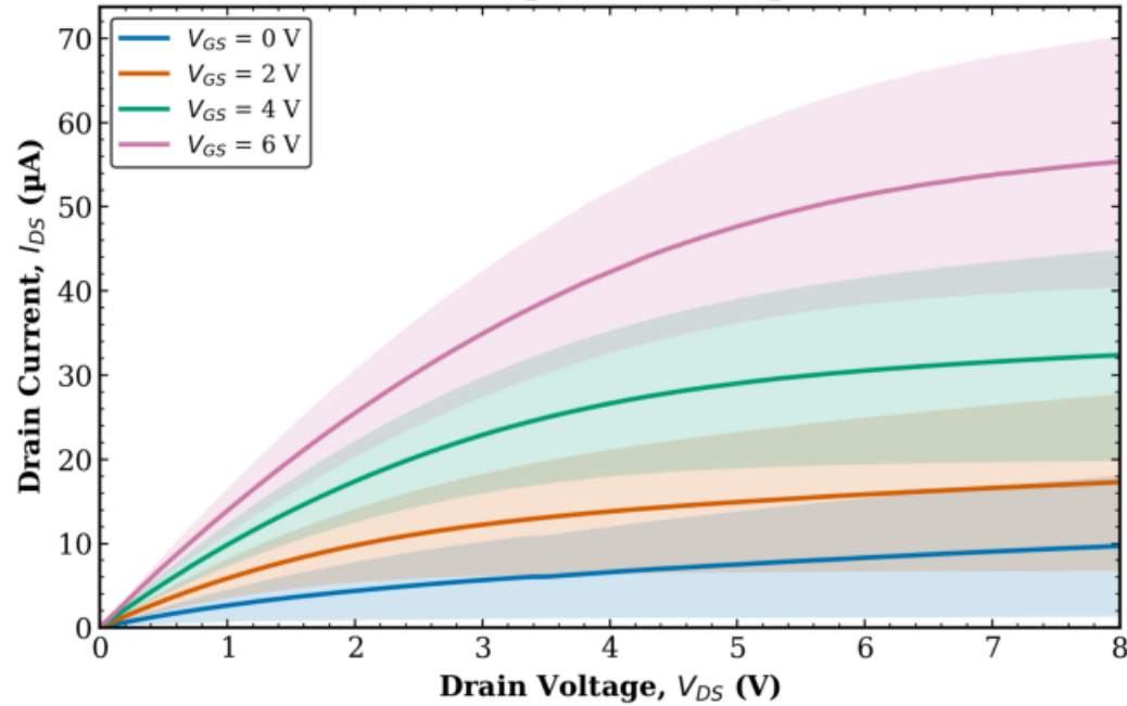
TFT3 Combined (Tr. 1 & 2) L = 20 \mu\text{m} , W = 50 \mu\text{m}
