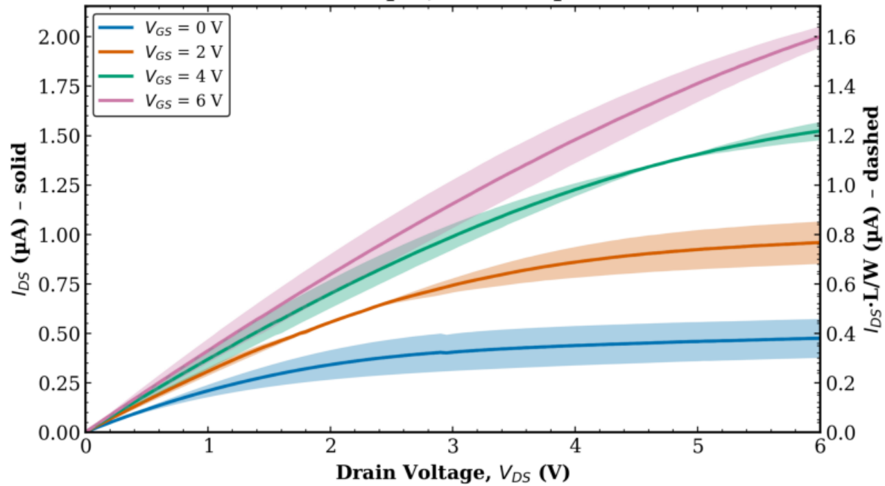
TFT3 Combined (Tr. 1 & 2) L = 8 \mu\text{m} , W = 10 \mu\text{m}
