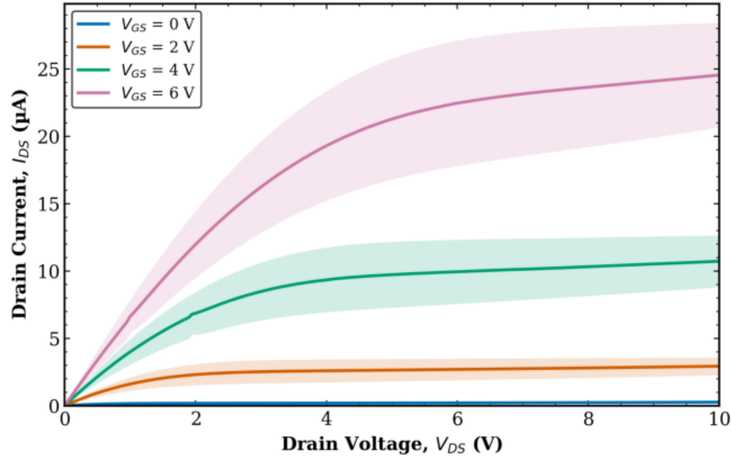
TFT3 Combined (Tr. 1 & 2) L = 40 \mu\text{m} , W = 100 \mu\text{m}
