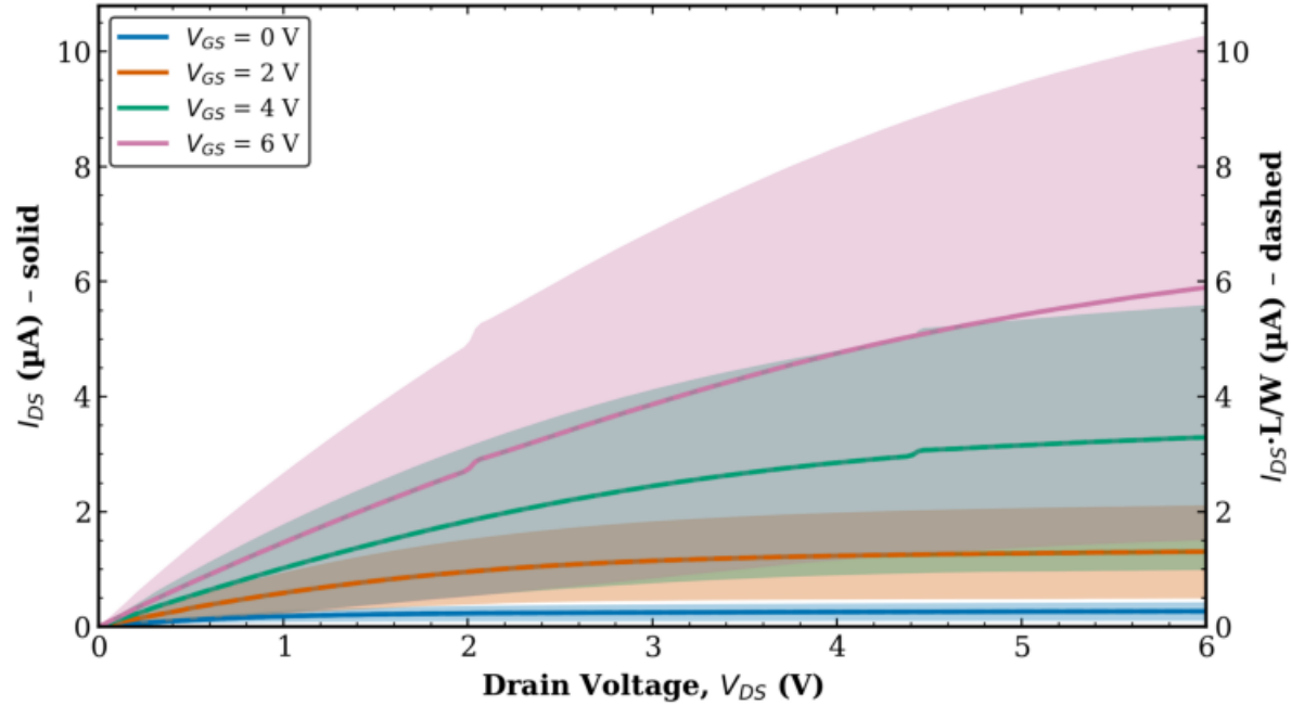
TFT3 Combined (Tr. 1 & 2) L = 10 \mu\text{m} , W = 10 \mu\text{m}
