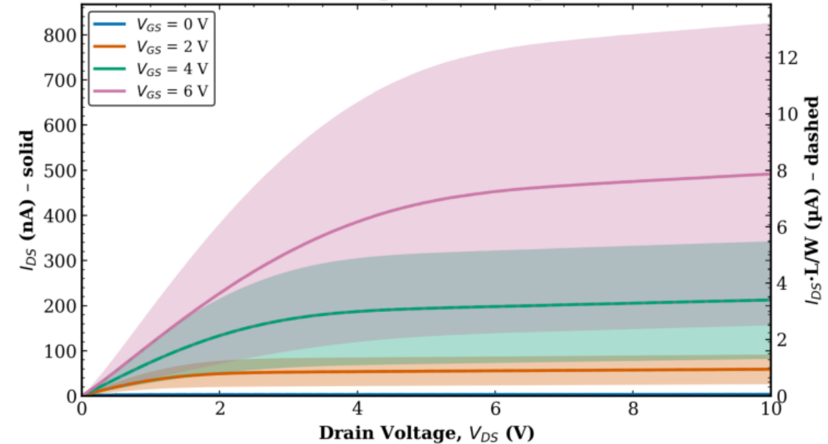
TFT3 Combined (Tr. 1 & 2) L = 160 \mu\text{m} , W = 10 \mu\text{m}
