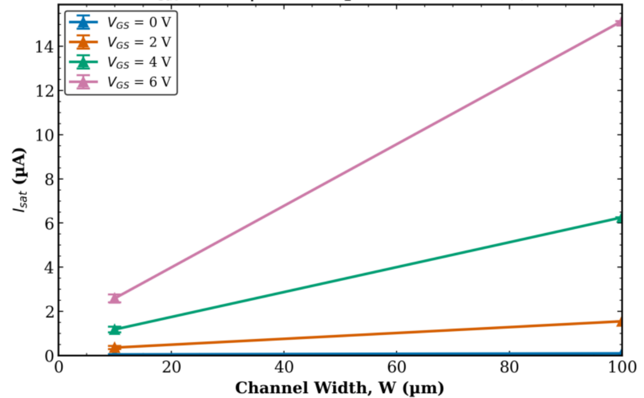
TFT3 Combined (Tr. 1 & 2) I_{sat} vs W | L = 80 \mu\text{m} (mean \pm std)
