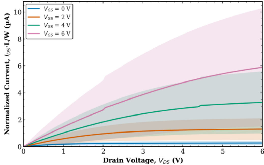
TFT3 Combined (Tr. 1 & 2) L = 10 \mu\text{m} , W = 10 \mu\text{m} (normalized)
