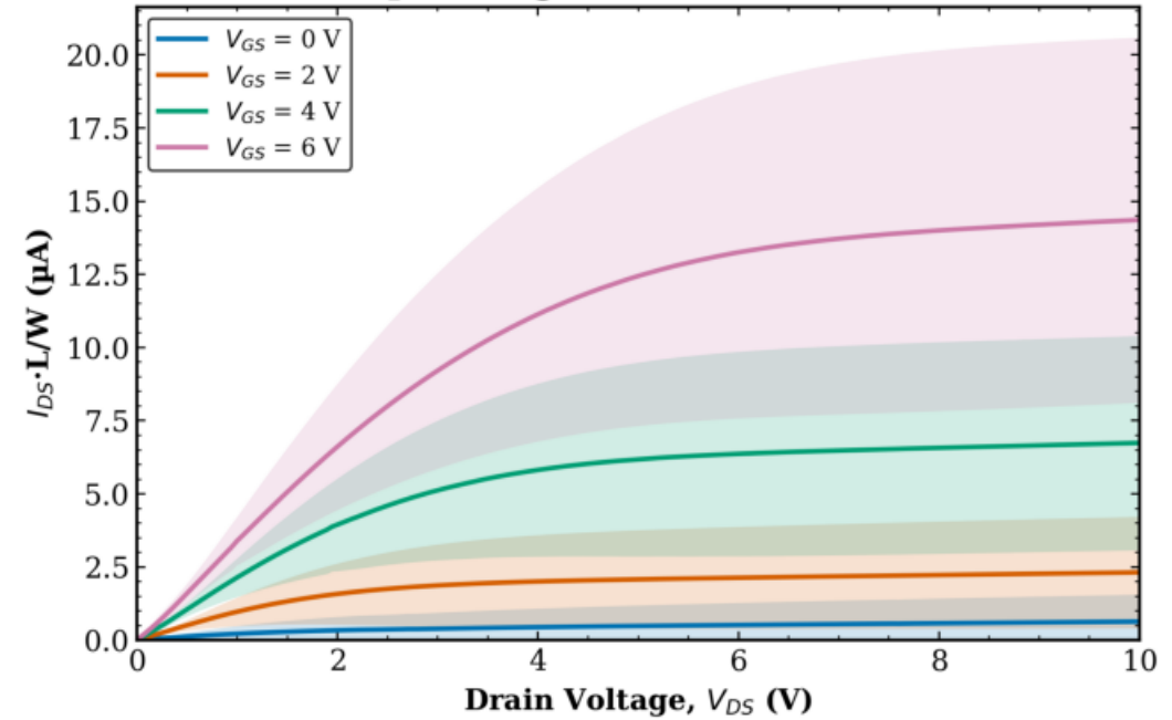
TFT3 Combined (Tr. 1 & 2) L = 40 \mu\text{m} - avg over all W (mean \pm std)
