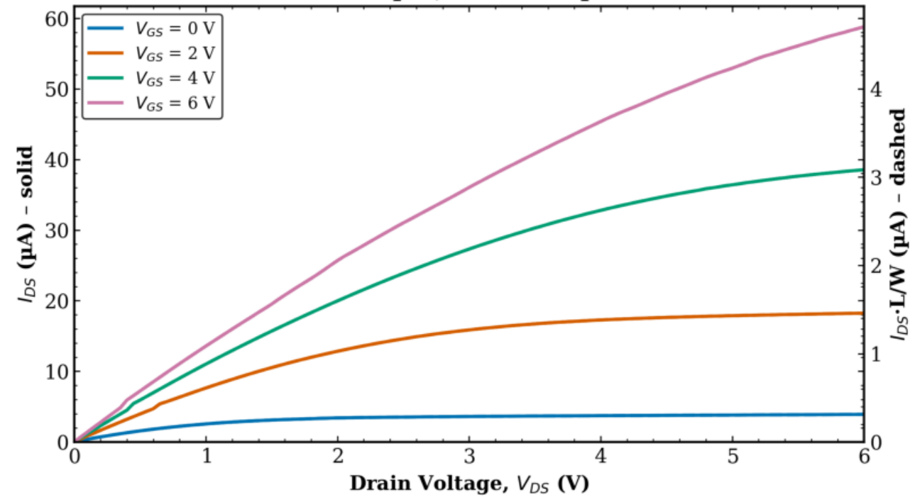
TFT3 Combined (Tr. 1 & 2) L = 8 \mu\text{m} , W = 100 \mu\text{m}
