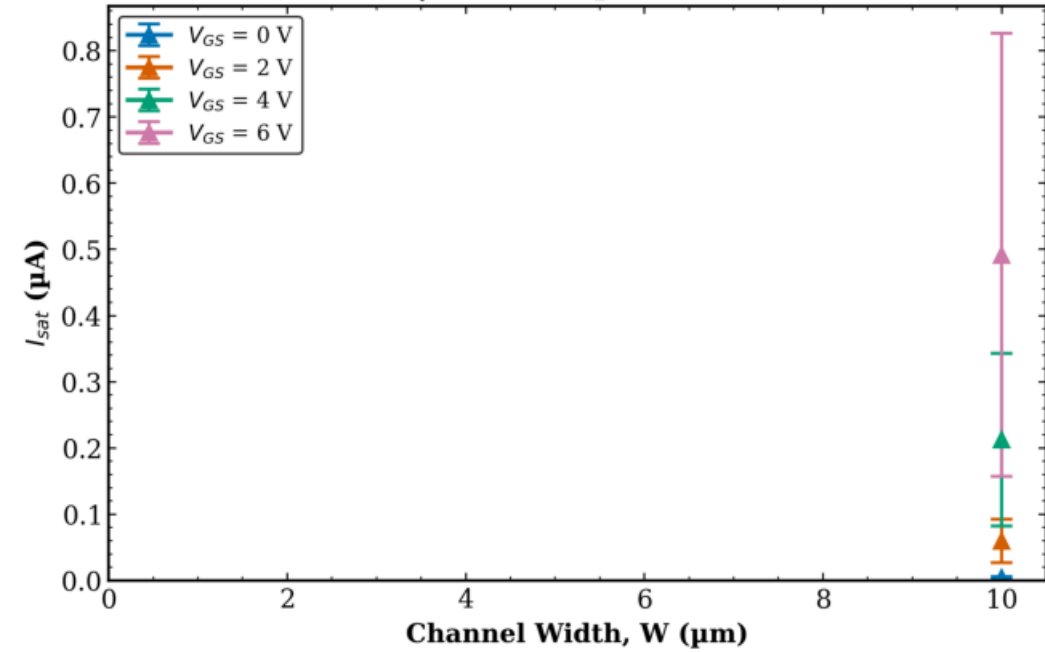
TFT3 Combined (Tr. 1 & 2) I_{sat} vs W | L = 160 μm (mean \pm std)
