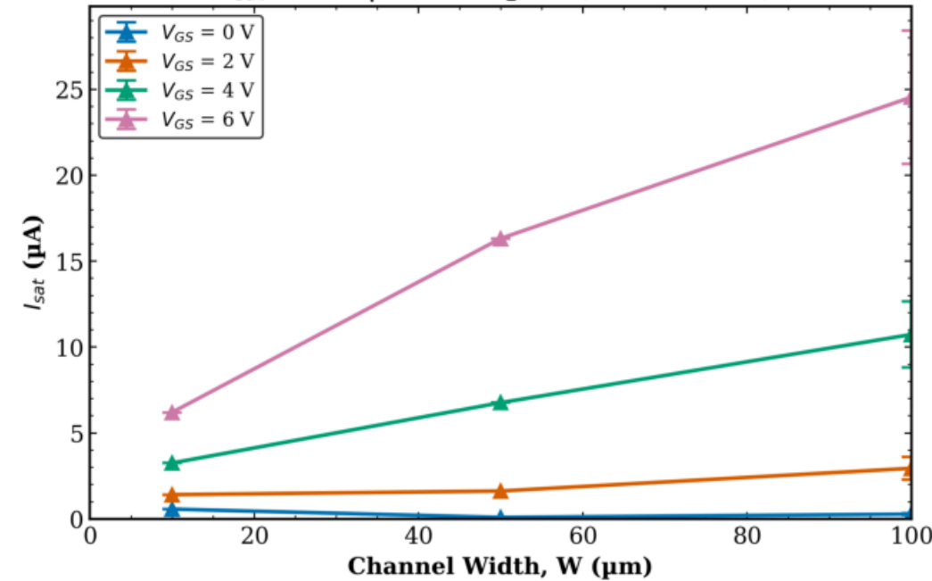
TFT3 Combined (Tr. 1 & 2) I_{sat} vs W | L = 40 μm (mean \pm std)
