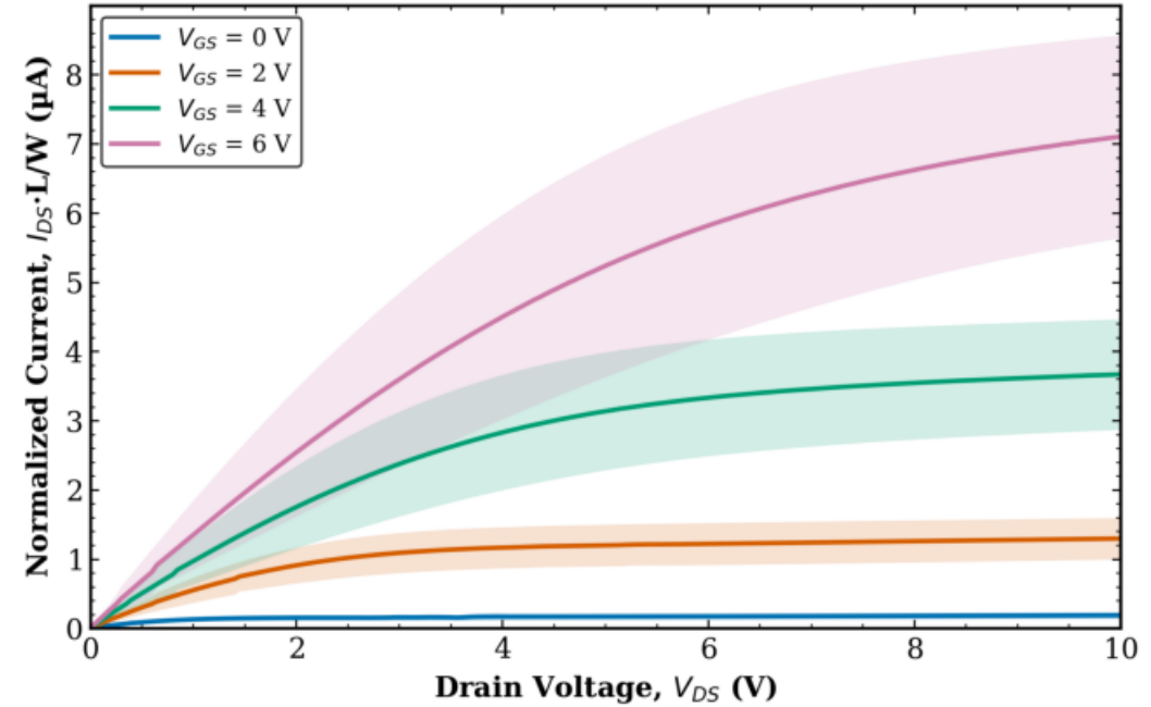
TFT3 Combined (Tr. 1 & 2) L = 10 \mu\text{m} , W = 100 \mu\text{m} (normalized)
