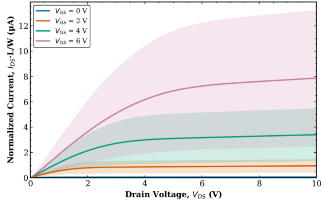
TFT3 Combined (Tr. 1 & 2) L = 160 \mu\text{m} , W = 10 \mu\text{m} (normalized)
