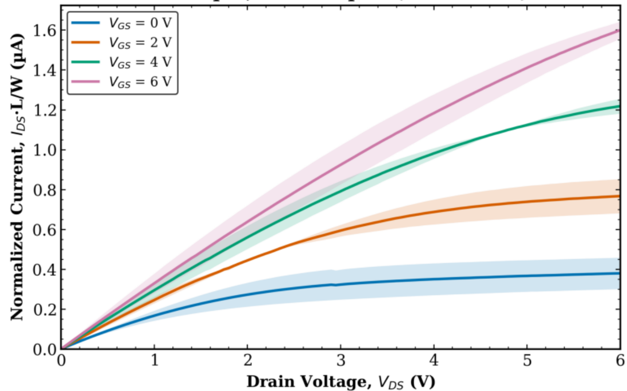
TFT3 Combined (Tr. 1 & 2) L = 8 \mu\text{m} , W = 10 \mu\text{m} (normalized)
