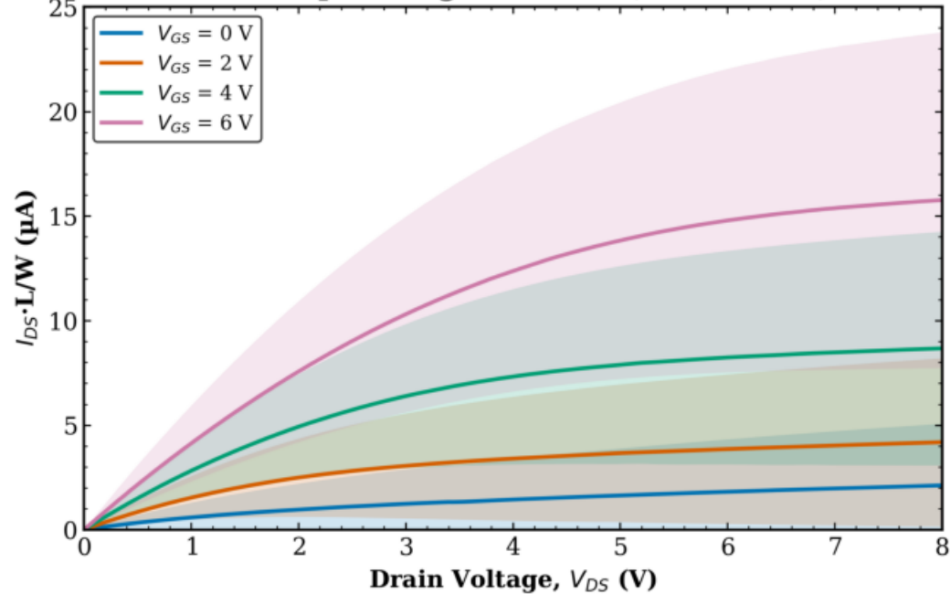
TFT3 Combined (Tr. 1 & 2) W = 50 \mu\text{m} - avg over all L (mean \pm std)
