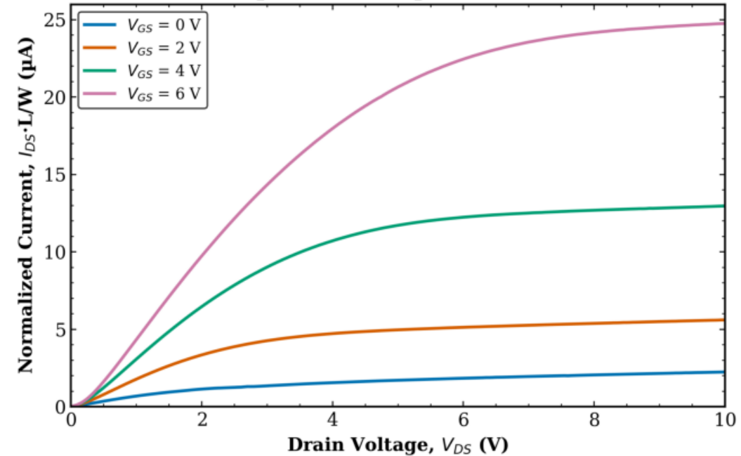
TFT3 Combined (Tr. 1 & 2) L = 40 \mu\text{m} , W = 10 \mu\text{m} (normalized)
