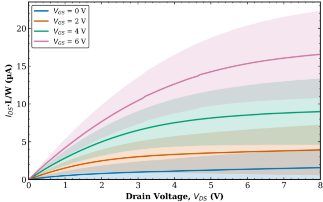
TFT3 Combined (Tr. 1 & 2) L = 20 \mu\text{m} - avg over all W (mean \pm std)
