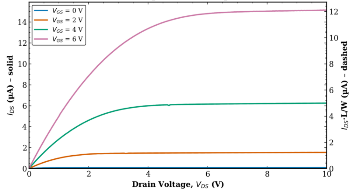
TFT3 Combined (Tr. 1 & 2) L = 80 \mu\text{m} , W = 100 \mu\text{m}
