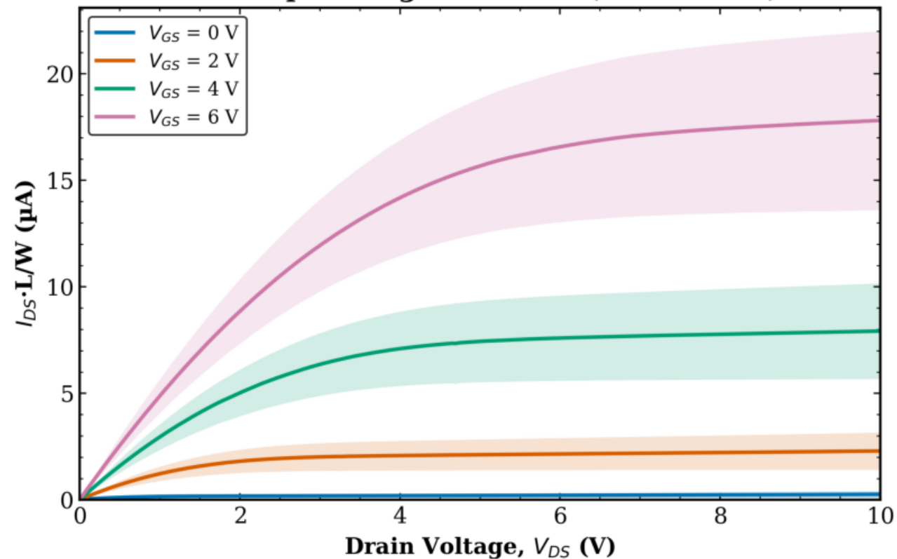
TFT3 Combined (Tr. 1 & 2) L = 80 \mu\text{m} - avg over all W (mean \pm std)
