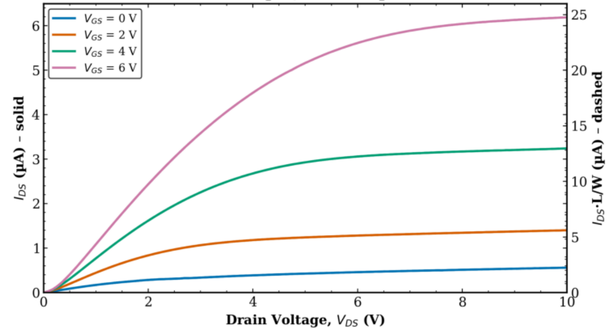
TFT3 Combined (Tr. 1 & 2) L = 40 \mu\text{m} , W = 10 \mu\text{m}
