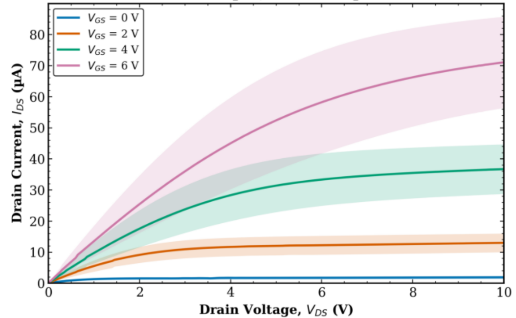
TFT3 Combined (Tr. 1 & 2) L = 10 \mu\text{m} , W = 100 \mu\text{m}
