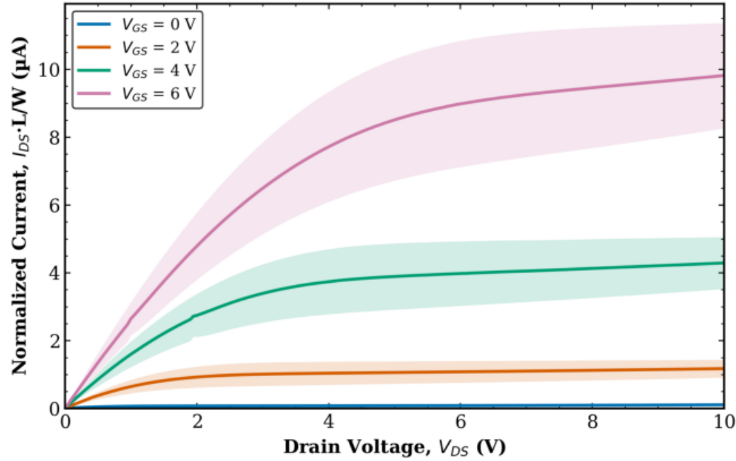
TFT3 Combined (Tr. 1 & 2) L = 40 \mu\text{m} , W = 100 \mu\text{m} (normalized)
