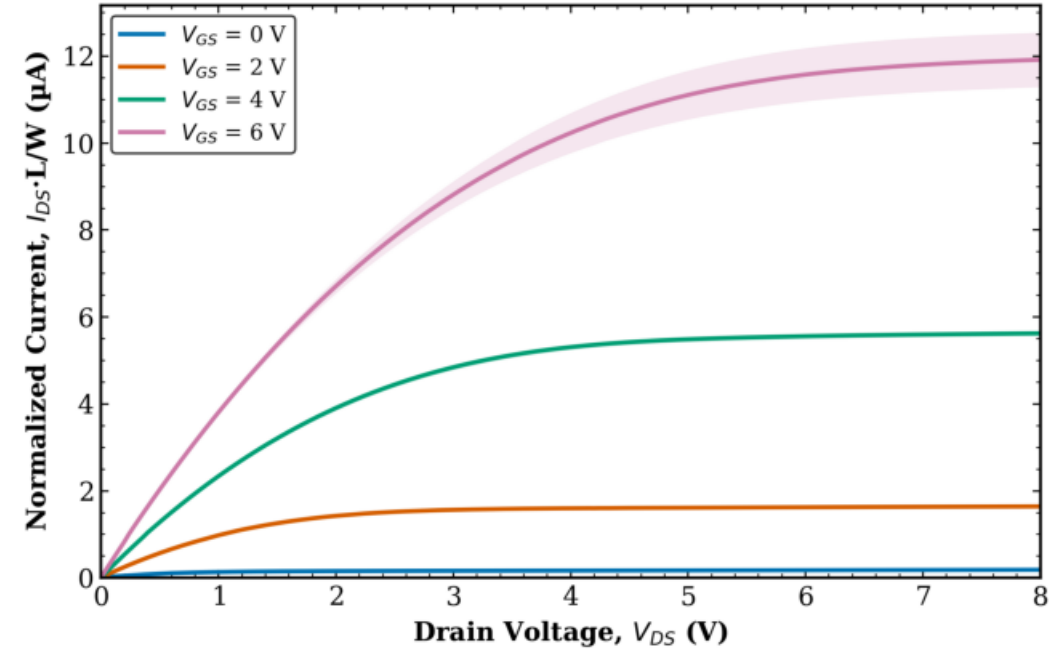
TFT3 Combined (Tr. 1 & 2) L = 20 \mu\text{m} , W = 100 \mu\text{m} (normalized)
