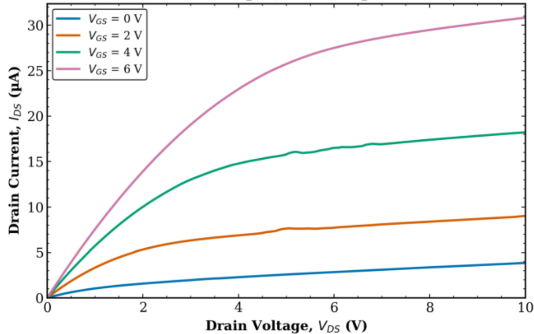
TFT3 Combined (Tr. 1 & 2) L = 10 \mu\text{m} , W = 50 \mu\text{m}
