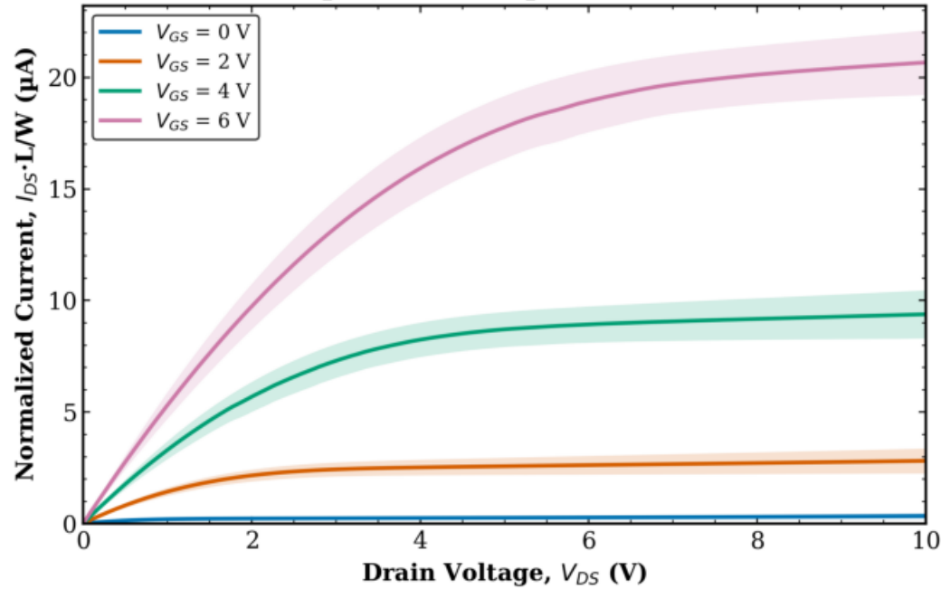
TFT3 Combined (Tr. 1 & 2) L = 80 \mu\text{m} , W = 10 \mu\text{m} (normalized)
