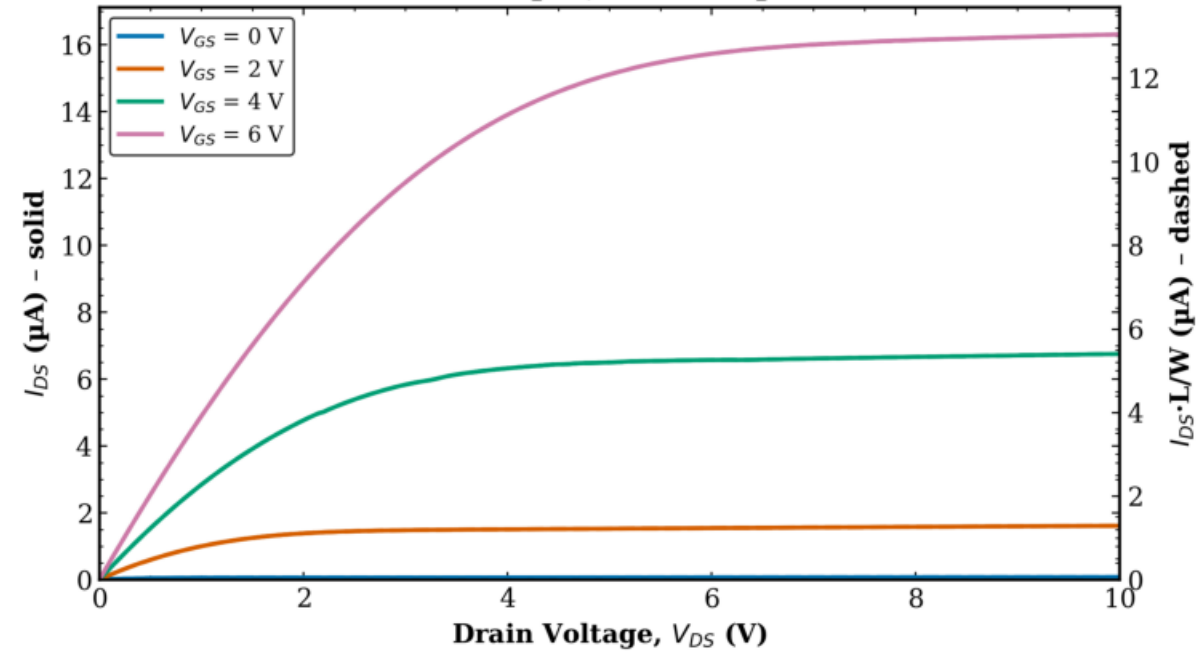
TFT3 Combined (Tr. 1 & 2) L = 40 \mu\text{m} , W = 50 \mu\text{m}
