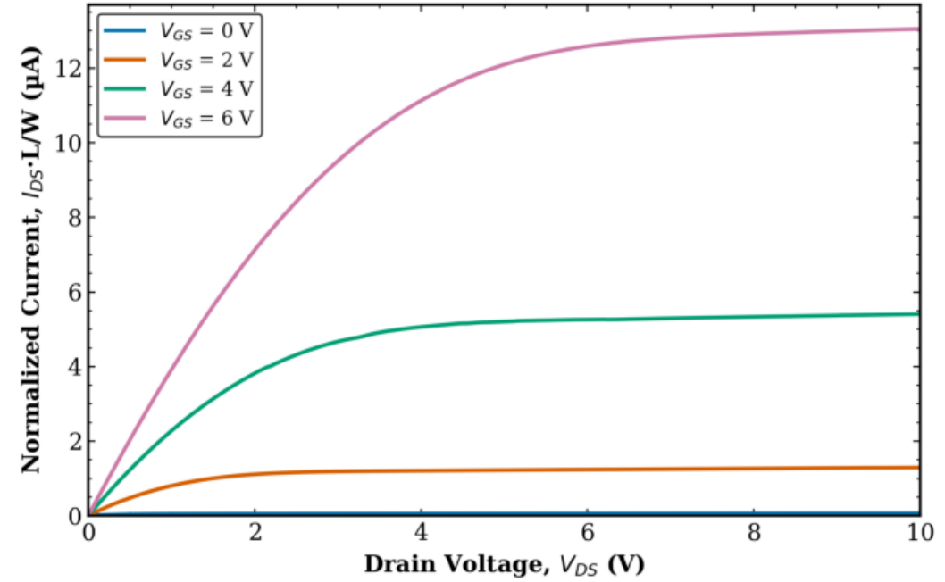
TFT3 Combined (Tr. 1 & 2) L = 40 \mu\text{m} , W = 50 \mu\text{m} (normalized)
