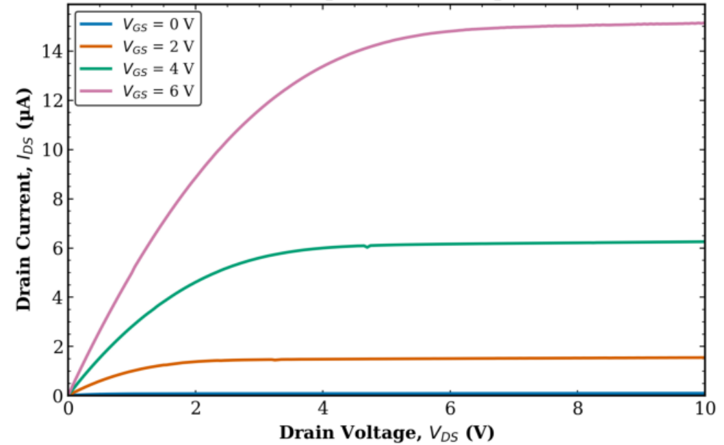
TFT3 Combined (Tr. 1 & 2) L = 80 \mu\text{m} , W = 100 \mu\text{m}
