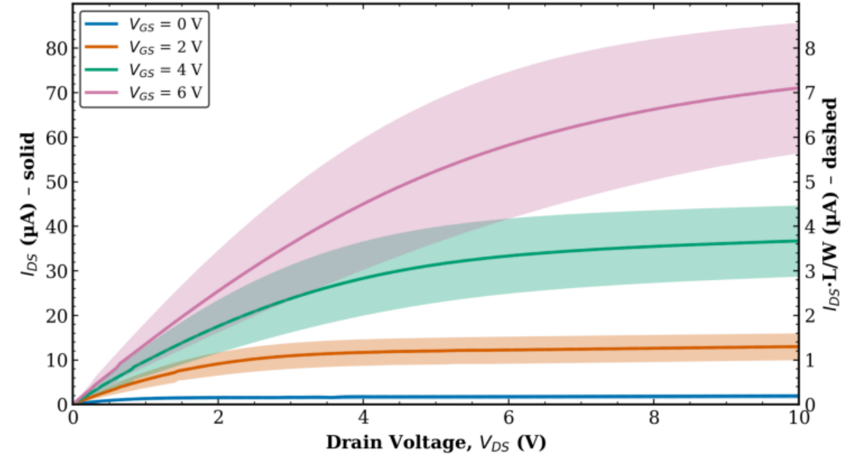
TFT3 Combined (Tr. 1 & 2) L = 10 \mu\text{m} , W = 100 \mu\text{m}
