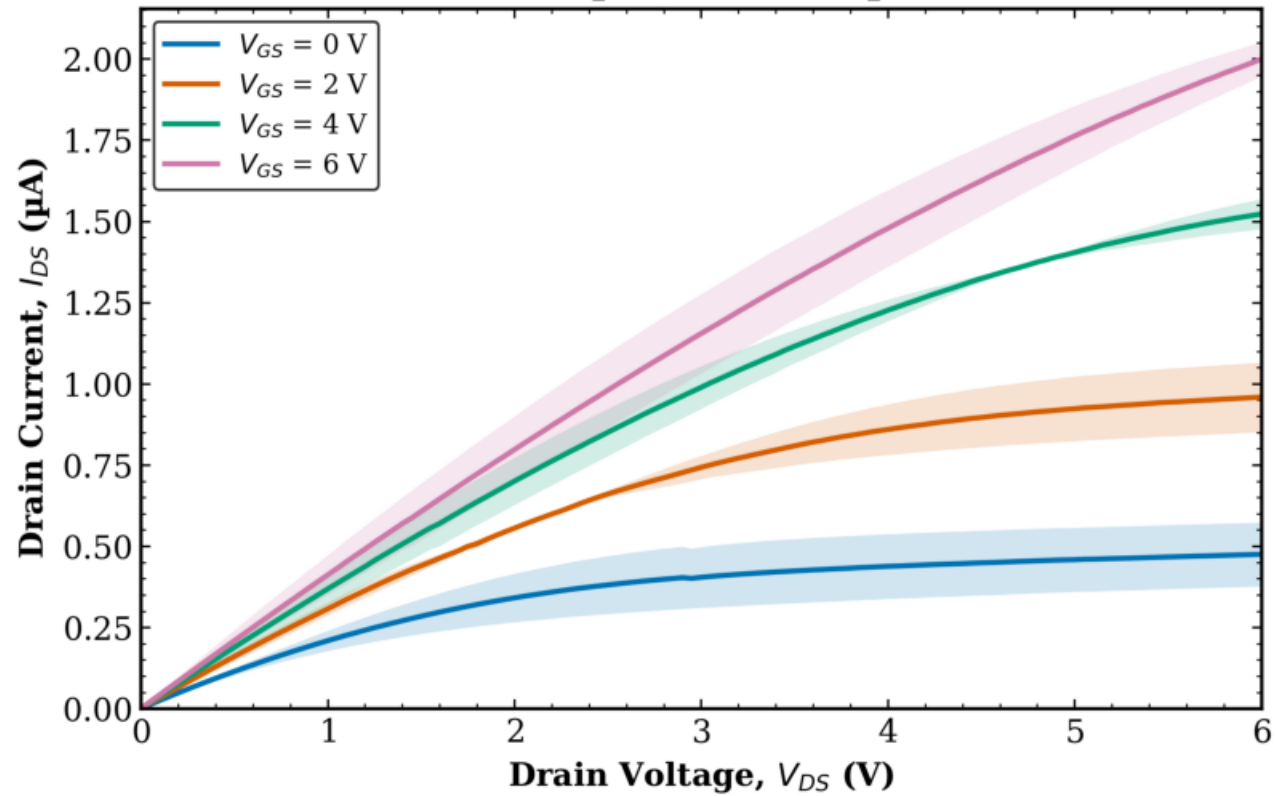
TFT3 Combined (Tr. 1 & 2) L = 8 \mu\text{m} , W = 10 \mu\text{m}
