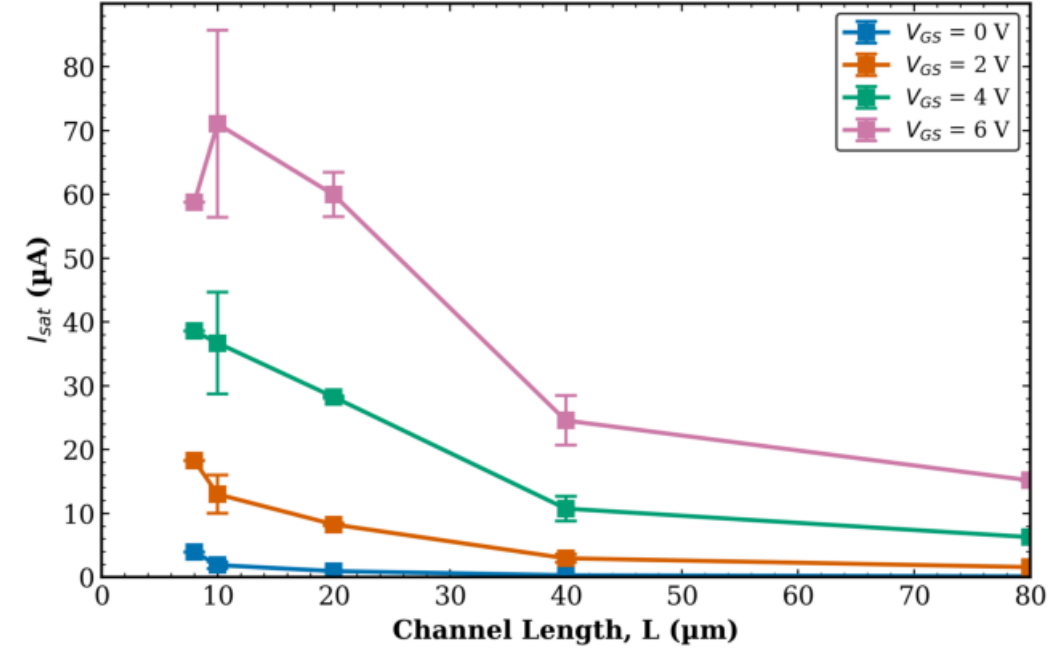
TFT3 Combined (Tr. 1 & 2) I_{sat} vs L | W = 100 \mu\text{m} (mean \pm std)
