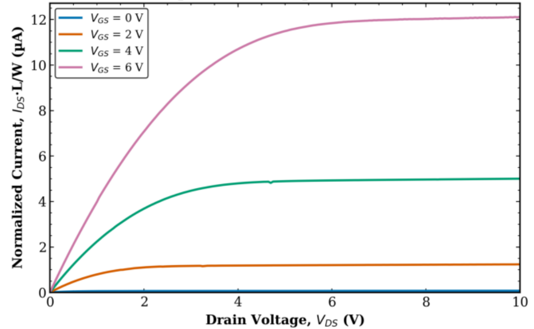
TFT3 Combined (Tr. 1 & 2) L = 80 \mu\text{m} , W = 100 \mu\text{m} (normalized)
