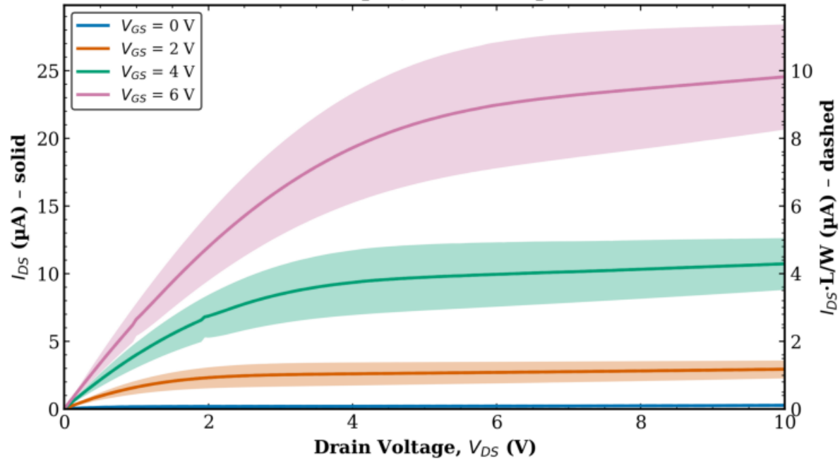
TFT3 Combined (Tr. 1 & 2) L = 40 \mu\text{m} , W = 100 \mu\text{m}
