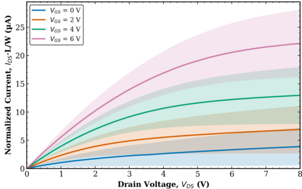
TFT3 Combined (Tr. 1 & 2) L = 20 \mu\text{m} , W = 50 \mu\text{m} (normalized)
