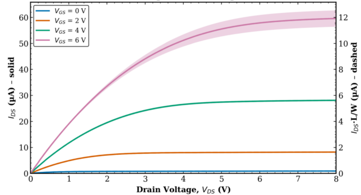
TFT3 Combined (Tr. 1 & 2) L = 20 \mu\text{m} , W = 100 \mu\text{m}
