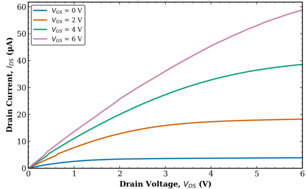
TFT3 Combined (Tr. 1 & 2) L = 8 \mu\text{m} , W = 100 \mu\text{m}
