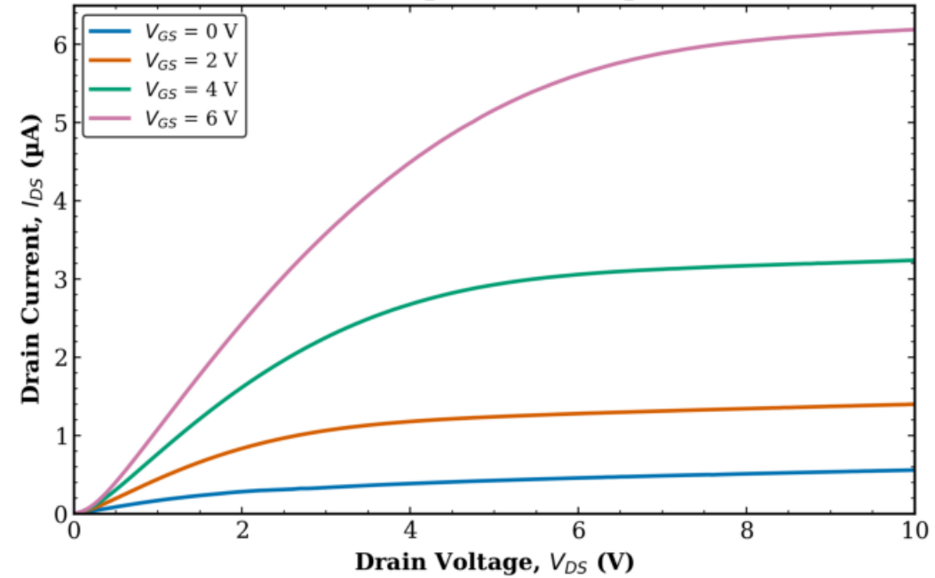
TFT3 Combined (Tr. 1 & 2) L = 40 \mu\text{m} , W = 10 \mu\text{m}
