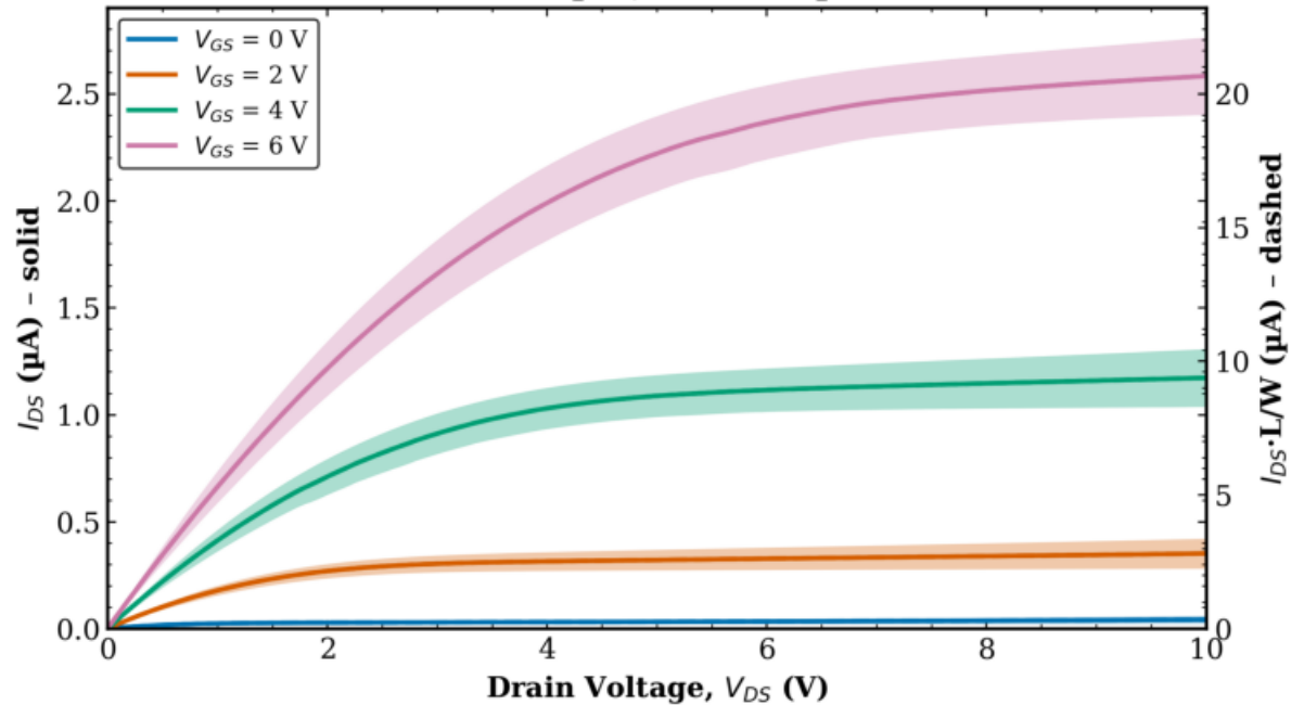
TFT3 Combined (Tr. 1 & 2) L = 80 \mu\text{m} , W = 10 \mu\text{m}
