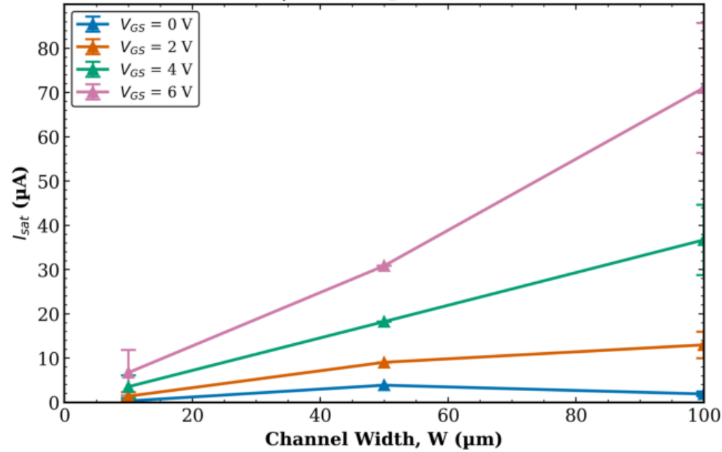
TFT3 Combined (Tr. 1 & 2) I_{sat} vs W | L = 10 \mu\text{m} (mean \pm std)
