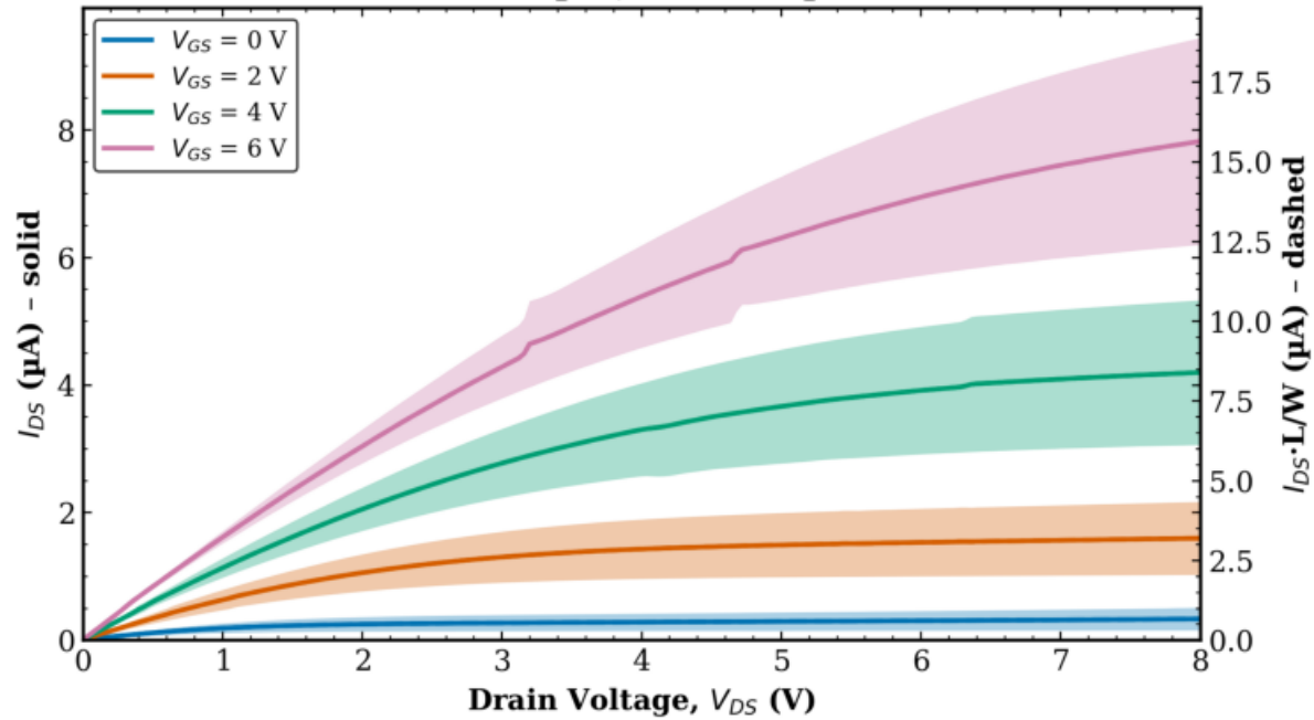
TFT3 Combined (Tr. 1 & 2) L = 20 \mu\text{m} , W = 10 \mu\text{m}
