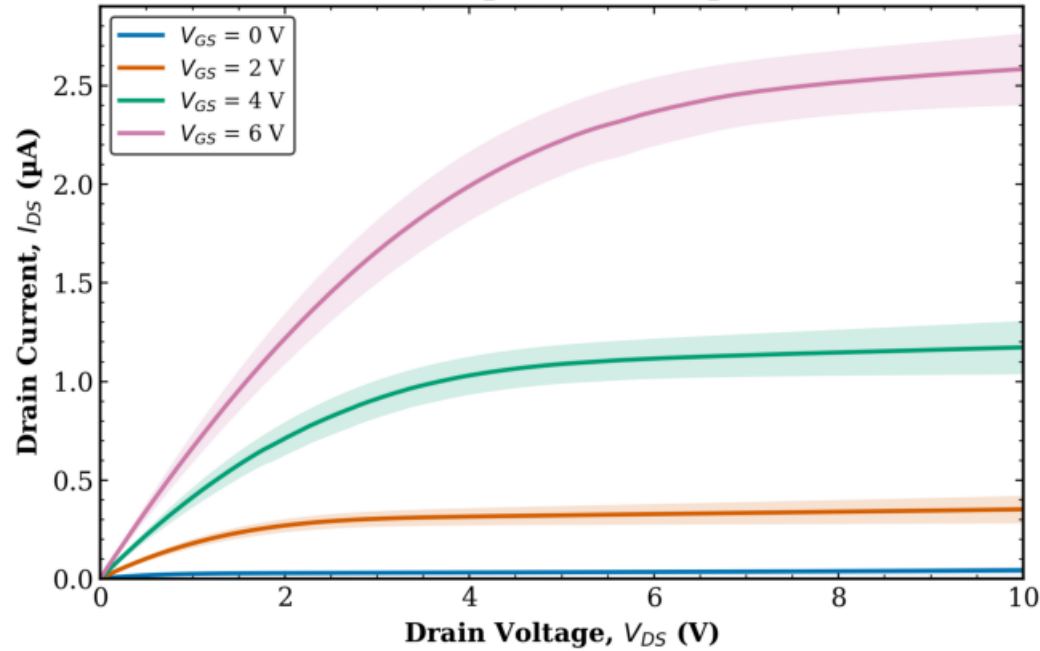
TFT3 Combined (Tr. 1 & 2) L = 80 \mu\text{m} , W = 10 \mu\text{m}
