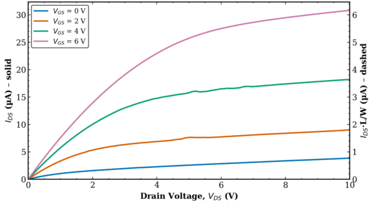
TFT3 Combined (Tr. 1 & 2) L = 10 \mu\text{m} , W = 50 \mu\text{m}
