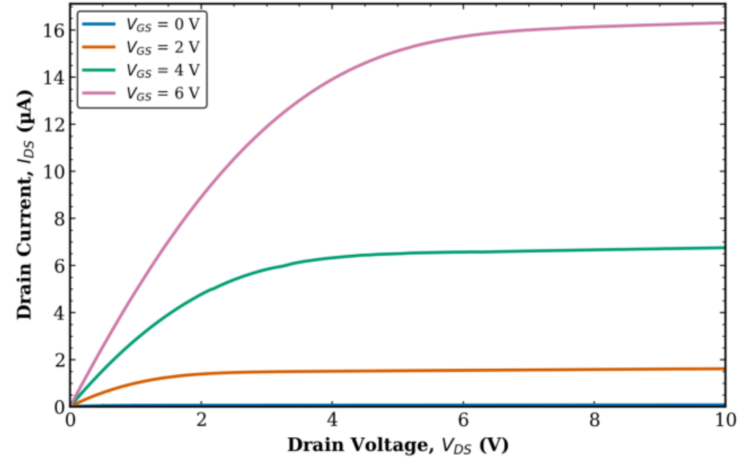
TFT3 Combined (Tr. 1 & 2) L = 40 \mu\text{m} , W = 50 \mu\text{m}
