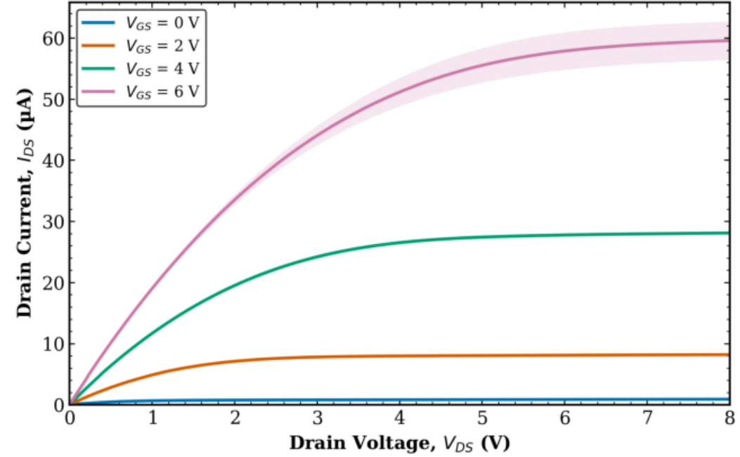
TFT3 Combined (Tr. 1 & 2) L = 20 \mu\text{m} , W = 100 \mu\text{m}
