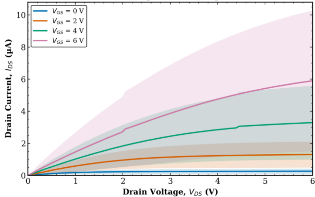
TFT3 Combined (Tr. 1 & 2) L = 10 \mu\text{m} , W = 10 \mu\text{m}
