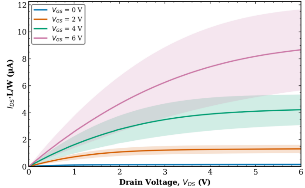
TFT3 Combined (Tr. 1 & 2) W = 100 \mu\text{m} - avg over all L (mean \pm std)
