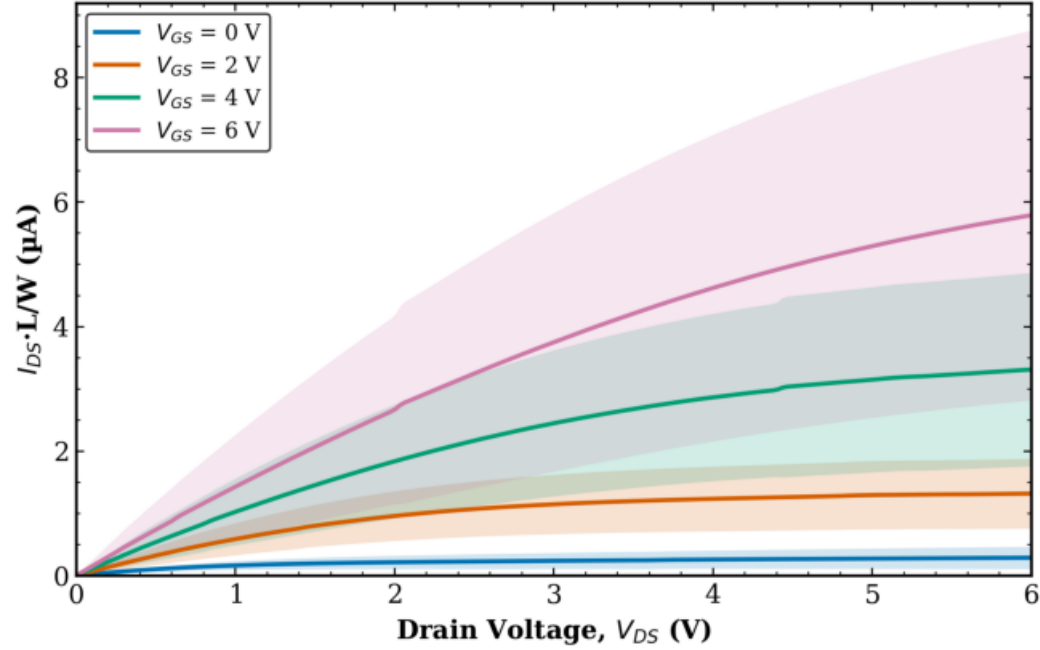
TFT3 Combined (Tr. 1 & 2) L = 10 \mu\text{m} - avg over all W (mean \pm std)
