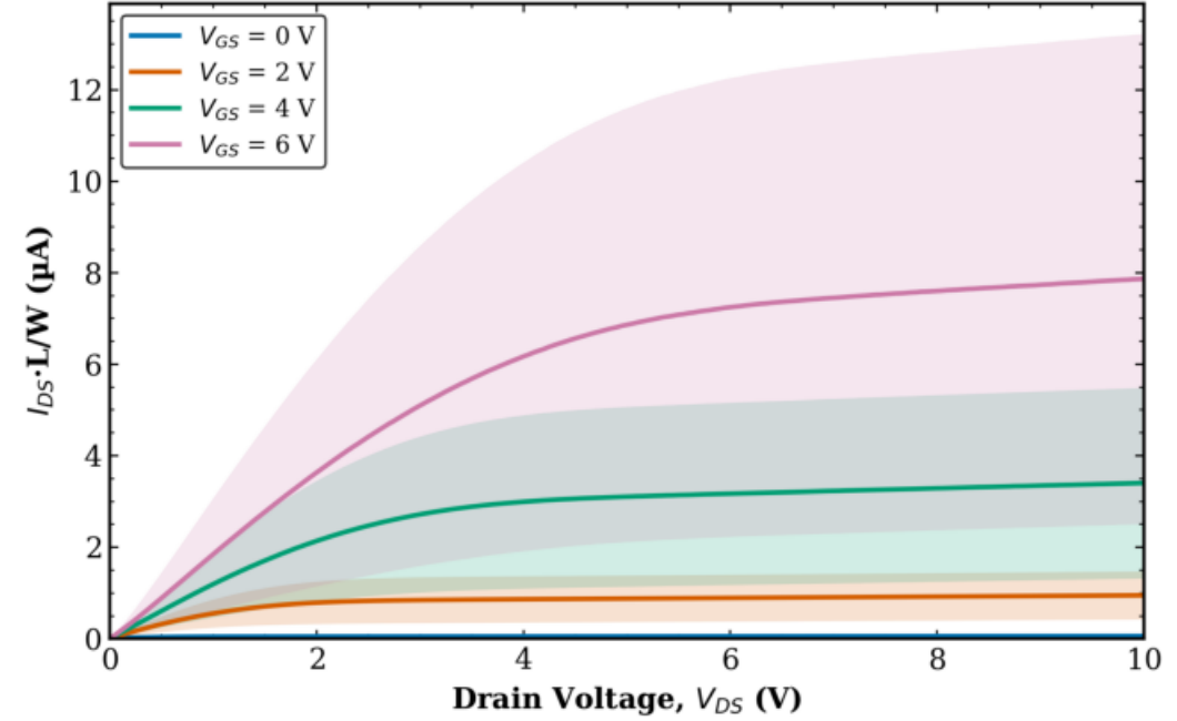
TFT3 Combined (Tr. 1 & 2) L = 160 \mu\text{m} - avg over all W (mean \pm std)
