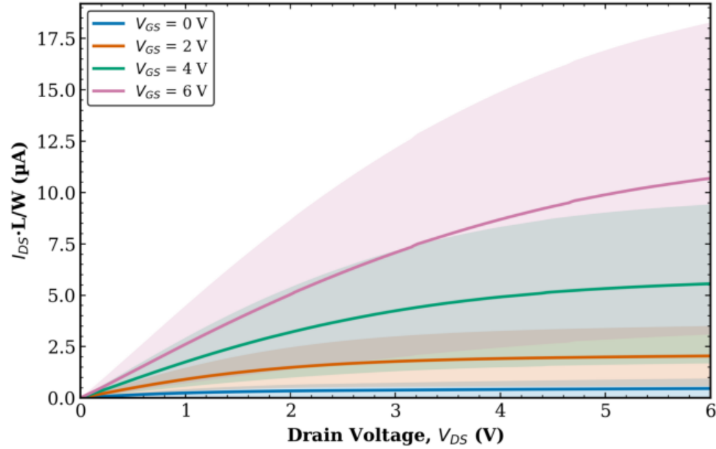
TFT3 Combined (Tr. 1 & 2) W = 10 \mu\text{m} - avg over all L (mean \pm std)
